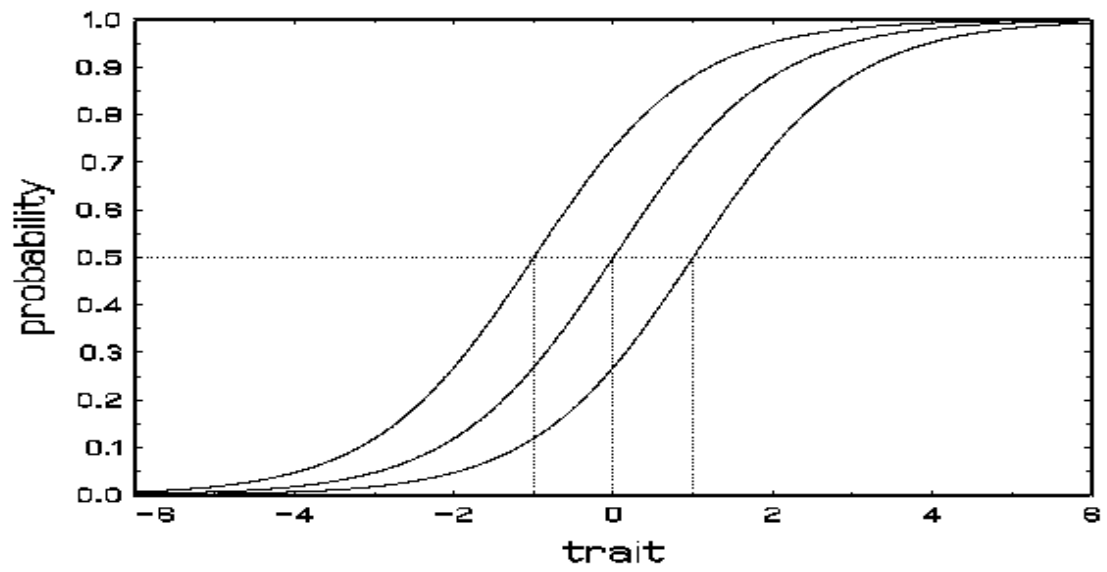
Figure 1. Rasch model with three items.
