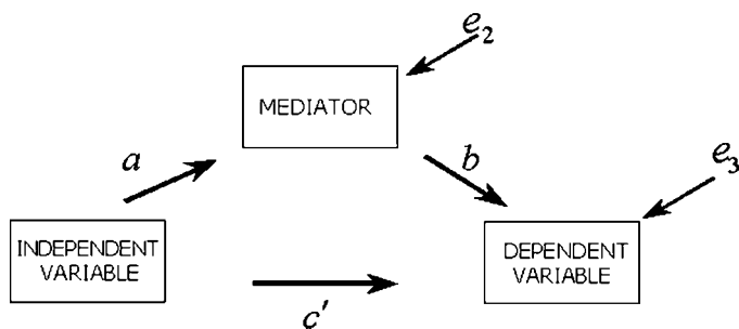
Figure 1 Mediation model.
