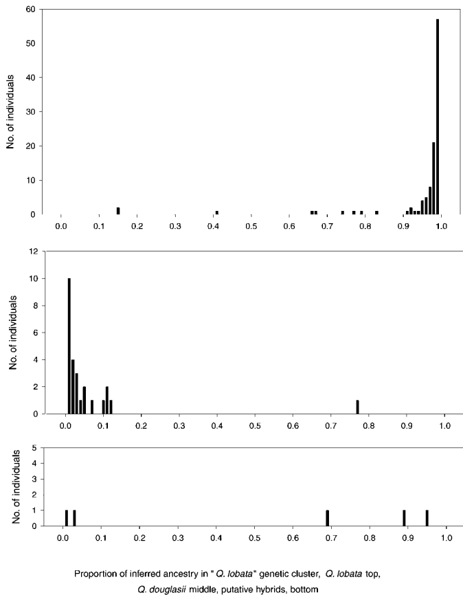
Fig. 5. Upper histogram shows the mean value of q_1^{(i)} (the proportion of ancestry in population 1, the “lobata” cluster) over a single run of the Gibbs sampler in structure for trees identified in the field as Quercus lobata . Middle histogram shows q_1^{(i)} for trees identified in the field as Q. douglasii . Lower histogram shows q_1^{(i)} for trees identified as putative hybrids based on intermediate morphology.
