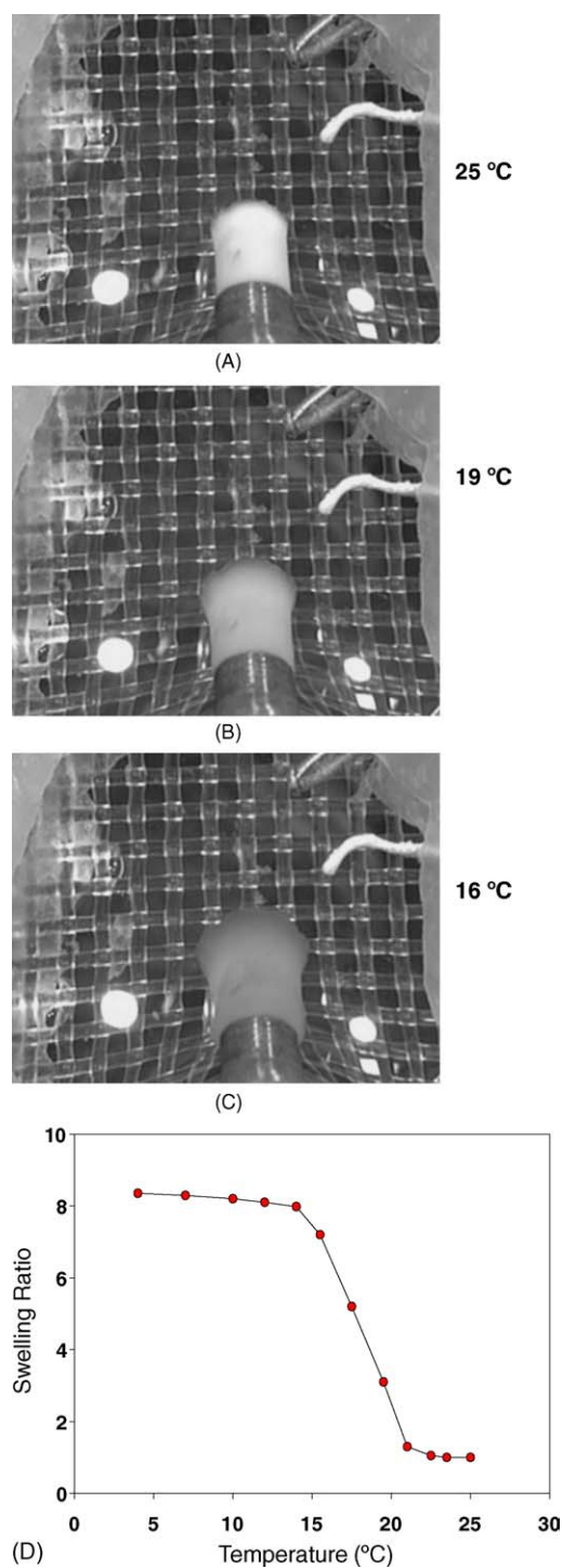
Fig. 2. (A) Image of hydrogel immersed in the recording chamber at approximately 25 °C. The nylon mesh within the chamber defined a grid of squares with center-to-center distance of approximately 0.95 mm. (B and C) Same hydrogel preparation, in the swollen state, at temperatures of approximately 19 and 16 °C, respectively. (D) Swelling curve. Swelling ratio for a representative (poly(NIPAAm-co-nBMA)) hydrogel as a function of temperature.
