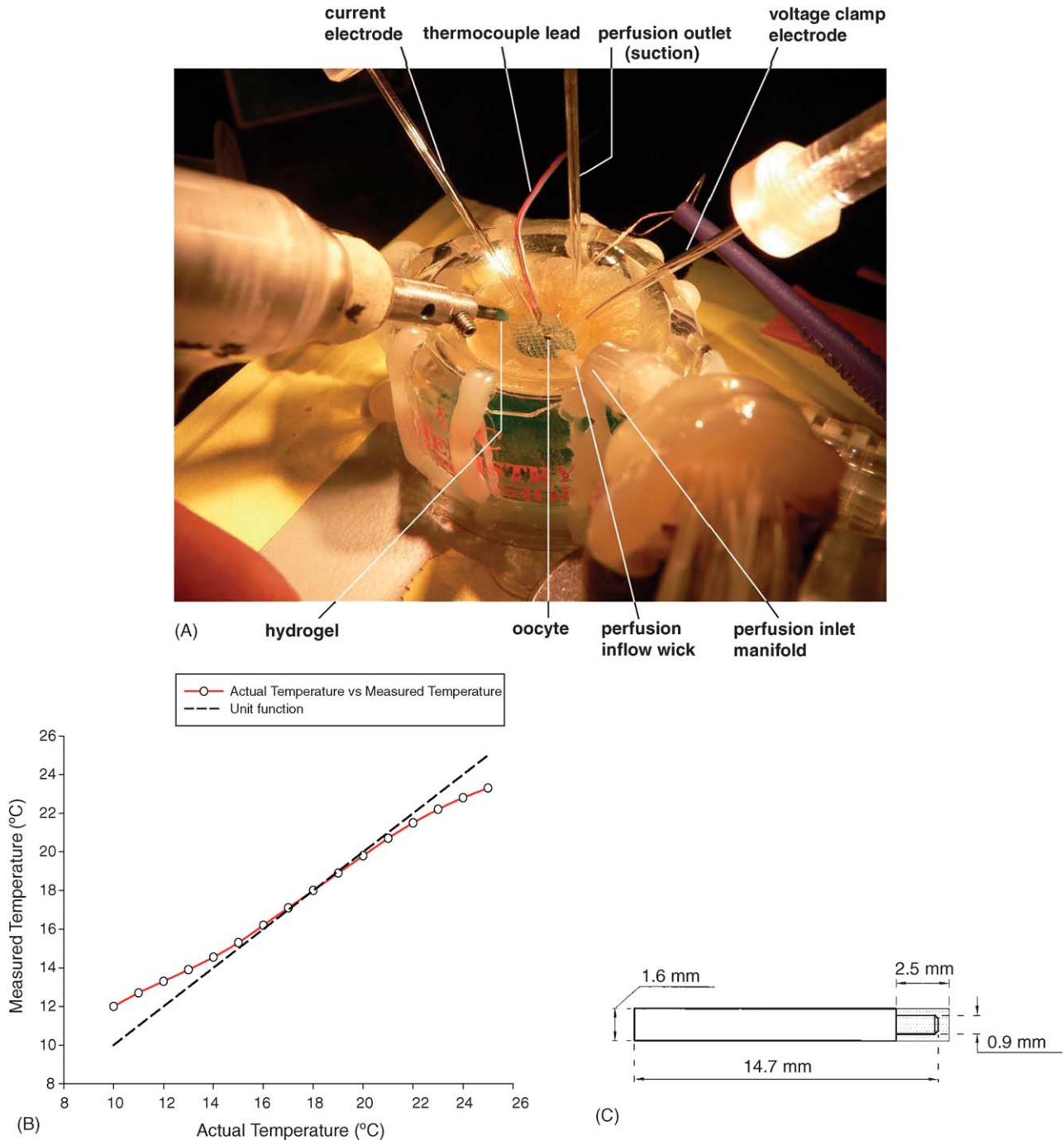
Fig. 1. Design and characteristics of recording chamber, and of the brass rod used to support the hydrogel. (A) Recording chamber, illustrating oocyte, electrodes for voltage clamp, and hydrogel. (B) Temperature calibration. Open circles show determinations of temperature reported by the thermocouple circuit (ordinate value) at a given bath temperature as measured by a calibrated thermometer (abscissa value). The dashed straight line is the unit function. (C) Schematic diagram of brass rod. Stipled region at the tip of the rod identifies the site of the hydrogel.
