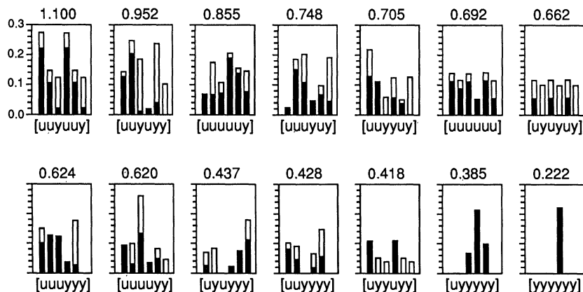
FIG. 2. Error spectra of the cyclic sets in lengths of six, as defined in text, within strain WMJ env , and mutation frequencies of cyclic sets (number on each box). Solid bar represents transition, and open bar represents transversion. The axis of ordinates refers to mutation frequency in each position.
