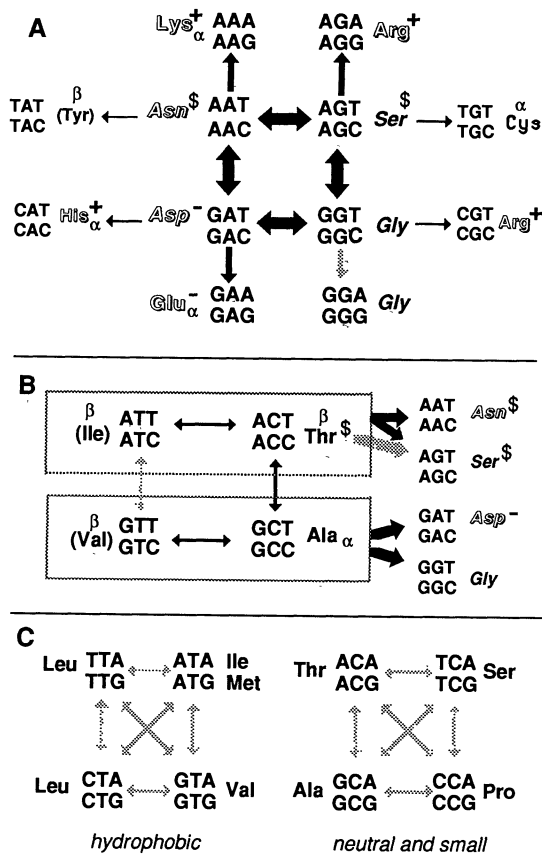
FIG. 4. Transition maps of amino acids caused by mutational hotspots in [uuyuyu] and [uuyuyu]. (A and B) Transition maps of amino acids encoded by uuy and uyy codons, produced by error spectra of the 6-mers of [uuyuyu] and [uuyuyu], respectively. (C) Transition map of amino acids encoded by uyu and yyu codons produced by mutations at the first letters. Solid arrows show nonsilent mutations or mutations that break or newly form potential glycosylation sites in the hypervariable regions; stippled arrow shows a silent mutation. The width of an arrow roughly indicates mutation frequencies. Amino acids in A and B are classified by the form of characters or by marks: amino acids shown in italics (Asn, Asp, Gly, and Ser) tend to form \beta -turns; amino acids marked with \alpha (Ala, Glu, His, Lys, and Cys) tend to form \alpha -helixes; amino acids marked with \beta (Ile, Thr, Tyr, and Val) tend to form \beta -sheets (18, 19). The amino acids shown by open characters (Arg, Asn, Asp, Glu, His, and Lys) are hydrophilic; amino acids in parentheses are hydrophobic; the others, except for cysteine, are neutral (20). $, amino acids that form potential glycosylation site; + and -, charge on amino acid.
