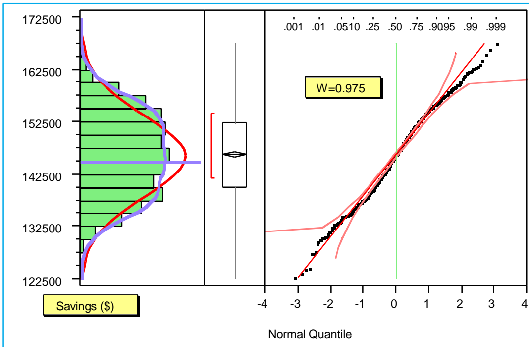
Figure 9a – Normal Quantile Plot of Saving
