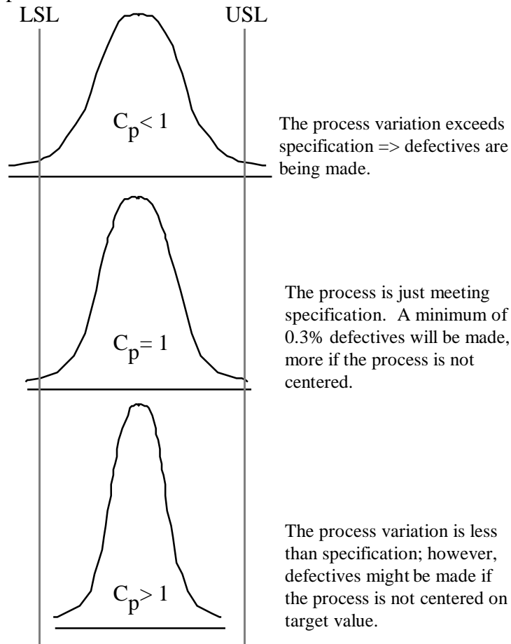
Figure 3 – Relationship Between Process Capability Index and Customer Specifications (Brassard and Ritter, 1994)
