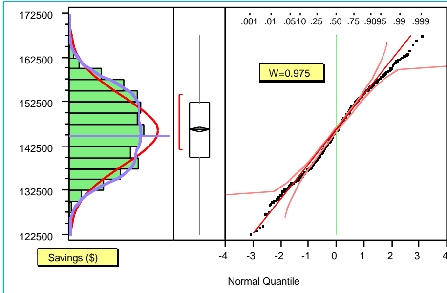
Figure 9a – Normal Quantile Plot of Saving
