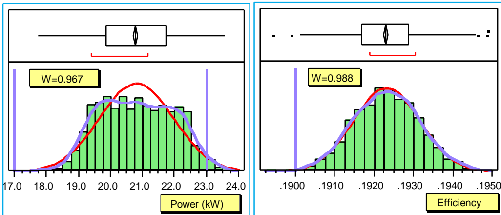
Figure 9b – Plots of Power and Efficiency
