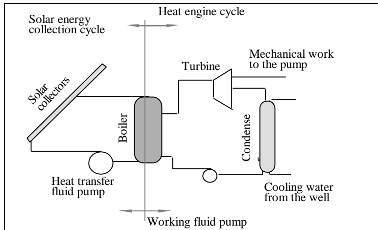
Figure 7 - Solar Powered Irrigation System
