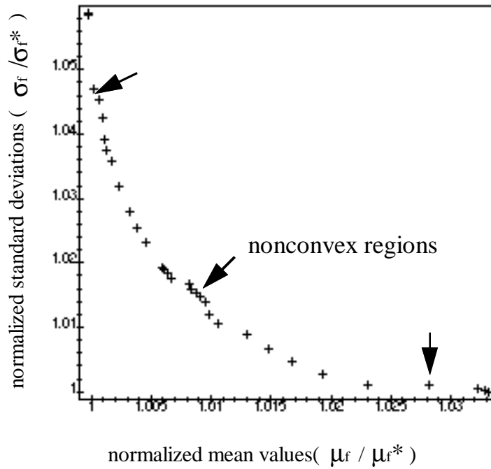
Figure 10 Efficient Solutions Using the CP Method (Two-Bar Problem)
