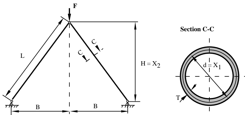
Figure 8 The Two-Bar Structure
