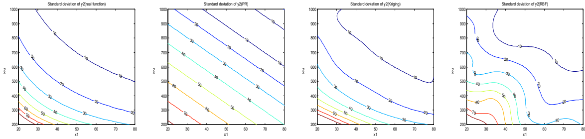
Figure A3 STD of Y_2 (large sample size)
