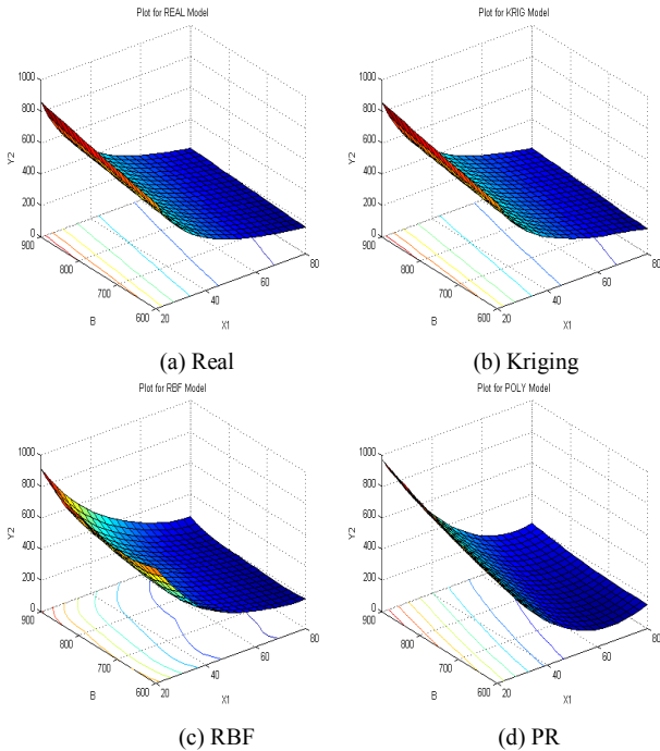
Figure 4 Comparisons of Metamodels of Y 2 (Large Sample Size)
