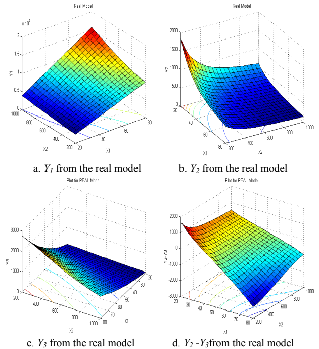
Figure 2. Behavior of the Real Performance
