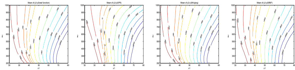
Figure A4 Means of Y_2-Y_3 (large sample size)
