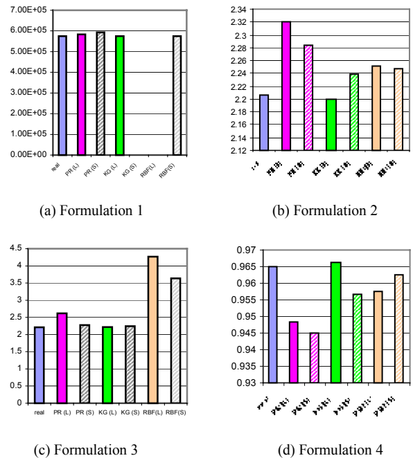
Figure 5. Comparison of Confirmed Objective Function Values
