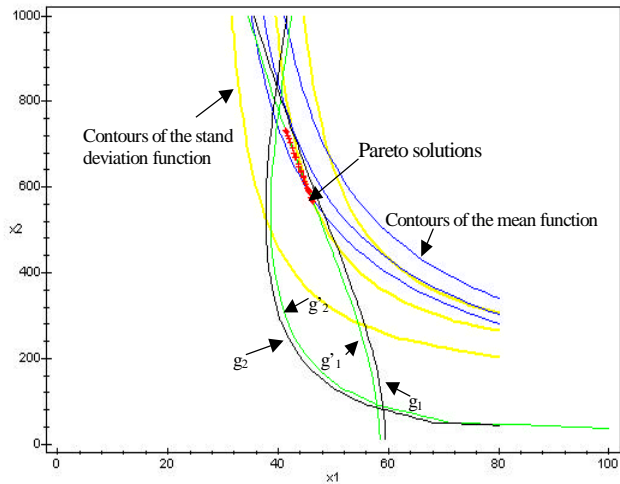
Figure 15 Pareto Solutions for the Two-Bar Robust Design Using the CP method
