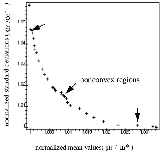
Figure 14 Efficient Solutions Using the CP Method (Two-Bar Problem)
