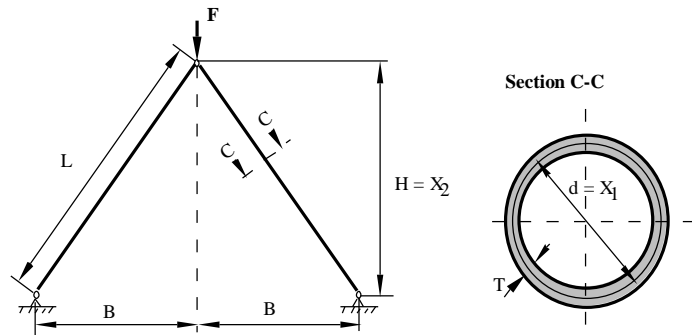
Figure 13. The Two-Bar Structure
