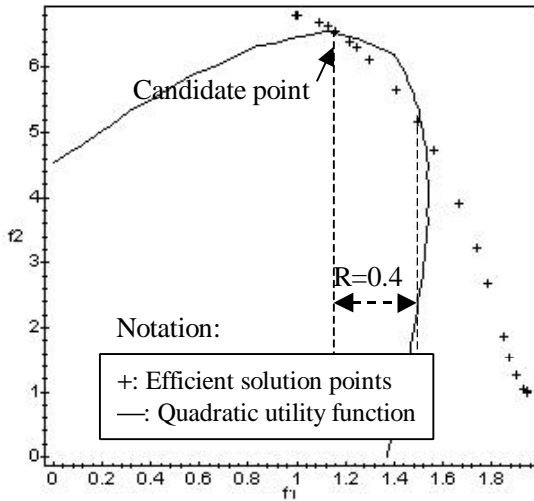
Figure 10 QUF Approximation (Scheme IV)
