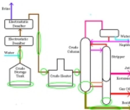
Figure 2: Another example of heavy organics deposition in petroleum refining
