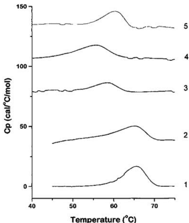
Fig. (4). DSC heating curves for the thermal denaturation of GLUT 1. Curve 1, No addition; curve 2, in the presence of 0.4 M NaCl; curve 3, in the presence of 4.8 mM ATP and 0.4 M NaCl; curve 4, in the presence of 4.8 mM ATP; curve 5, in the presence of 4.8 mM ATP and 500 mM D-glucose (Adapted from Fig. 3 of ref. [70]).
