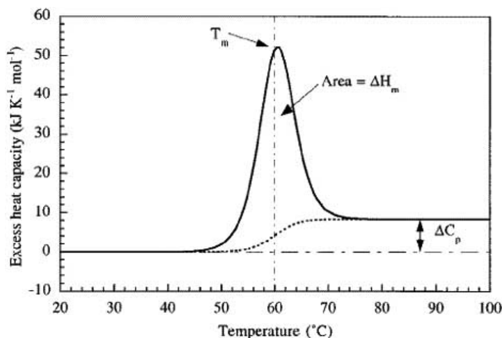
Fig. (1). DSC experiment for the two-state unfolding of a globular protein (Adapted from Fig. 1 of ref. [1]).
