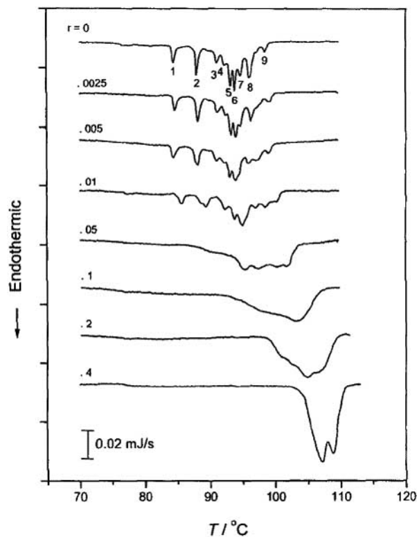
Fig. (8). DSC curves of ColE1 plasmid DNA in solutions of various distamycin concentrations. Distamycin concentration was indicated as r , the molar ratio of distamycin to base pairs of DNA (Adapted from Fig. 3 of ref. [88]).
