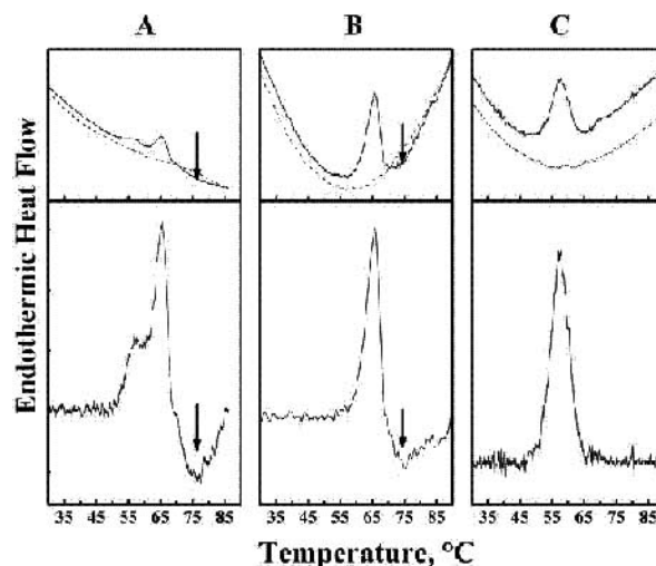
Fig. (2). DSC thermograms observed during the thermal unfolding of S. lividans xylanase A. The data are representative of the intact enzyme (A), the catalytic domain (B), and the xylan binding domain (C). The top panels show thermograms observed during the unfolding of the protein (solid lines) and those obtained in subsequent heating scans after complete suppression of all protein-related thermotropic events (broken line). The bottom panels show the unfolding thermograms after baseline subtraction. (Adapted from Fig. 1 of ref. [38]).
