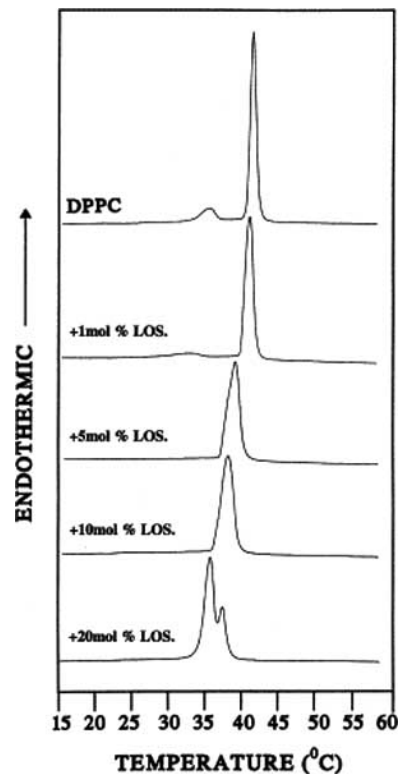
Fig. (7). Normalized DSC scans of DPPC bilayers containing losartan at different concentrations (Adapted from Fig. 2 of ref. [79]).
