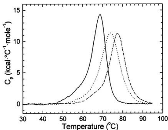
Fig. (9). DSC thermograms for the d(TGCT)-d(AGCA) unplatinated duplex (solid line) containing a single, site-specific interstrand cross-link of cisplatin (dot-dash line) or transplatin (dashed line). (Adapted from Fig. 2 of ref. [92]).
