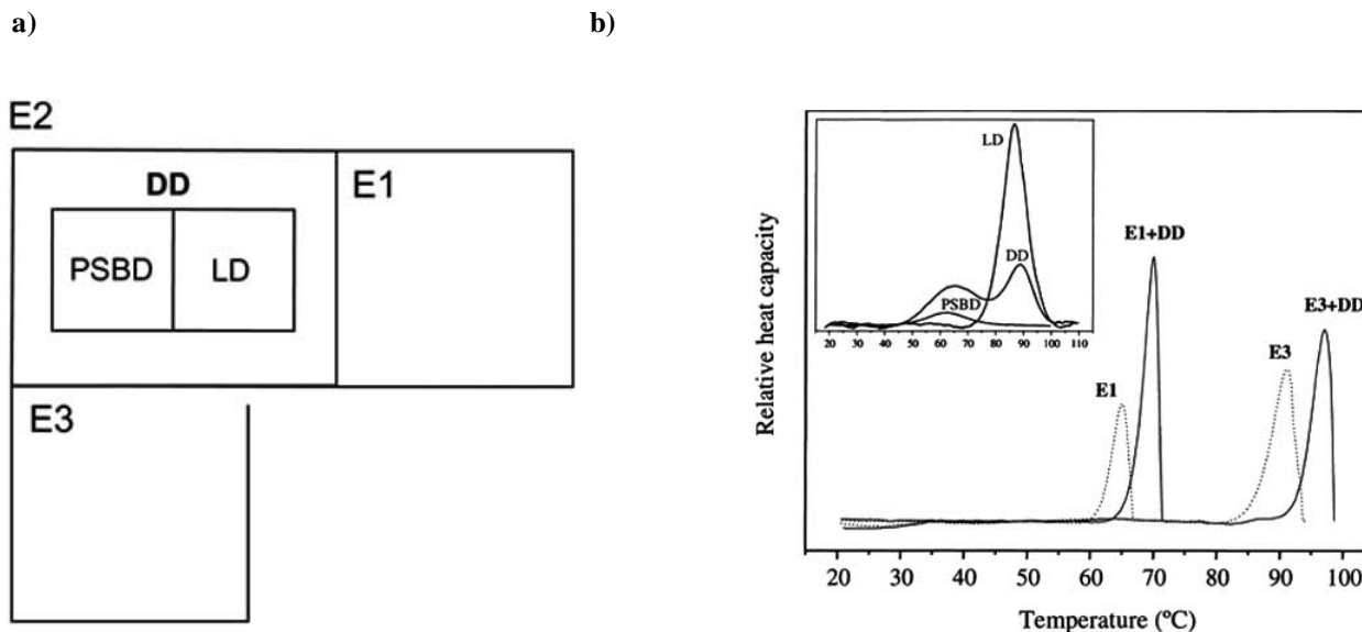
Fig. (6). a) Schematic arrangement of subunits of the pyruvate dehydrogenase multienzyme complex: E1=pyruvate decarboxylase, E2=diacyltransferase, E3=diacyl dehydrogenase, PSBD=peripheral subunit-binding domain, LD=lipoyl domain, DD= recombinant di-domain representing the LD and PSBD of E2; b) DSC trace of the thermal denaturation of E3 and E1 in the absence (dotted line) and presence (solid line) of PSBD (Adapted from Fig. 5 of ref. [77]).
