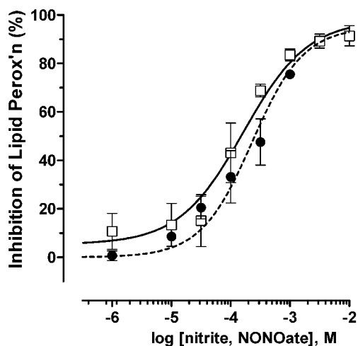
Figure 7. Comparison of NO donor with t -amyl nitrite. Inhibition of lipid peroxidation induced by \text{FeSO}_4 ( 50 \mu\text{M} ) as assessed by TBARS determination, on incubation of rat brain synaptosomes with: (a) IAN ( \square , solid line); and Sper/NO ( \bullet , dashed line). Percentage inhibition relative to: control TBARS in the presence of vehicle and absence of \text{FeSO}_4 (100%); TBARS in the presence of vehicle, adjuvant, and \text{FeSO}_4 (0%). Error bars show SEM ( n = 3 ). Data are fitted to sigmoidal curves ( \text{EC}_{50} : IAN = 1.6 \times 10^{-4} M; Sper/NO = 2.0 \times 10^{-4} M).
